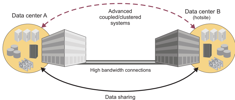
Figure 126. Tier 6: Synchronous replication with coupling or clustering applications
