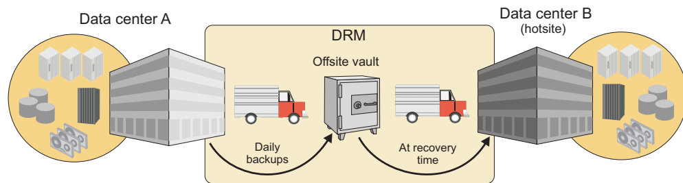
Figure 122. Tier 2: Offsite vaulting with a recovery site
